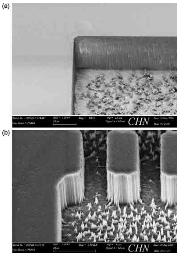
Fig. 3. Anisotropic etch profiles from (a) 55 μm thick parylene and (b) 10 μm thick parylene.
