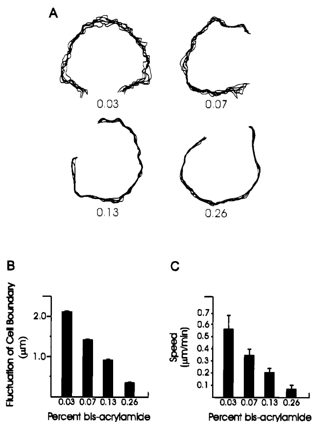
FIG. 2. Measurements of lamellipodial activity and cell motility on substrates of various flexibilities. ( A , B ) Fluctuation of the lamellipodia of NRK cells cultured on substrates of varying flexibilities. Numbers in A indicate the percentage concentration of bis-acrylamide. Images of cells were recorded every 2 min over a period of 10 min and active lamellipodia were traced and overlaid to generate the plots. The degree of lamellipodial protrusion/retraction was then quantified based on the SD of the position of seven randomly chosen points along the active edge. Fifteen cells were analyzed under each bis-acrylamide concentration ( B ). Lamellipodia become less active with increasing rigidity of the substrate. ( C ) Rate of locomotion of 3T3 cells on substrates of varying flexibilities. Cells become less motile with increasing rigidity of the substrate.
