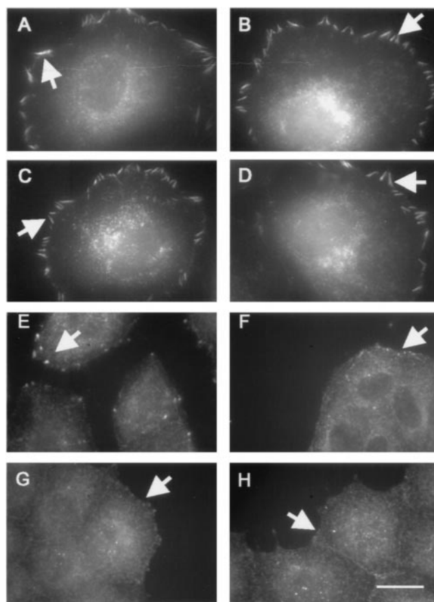
FIG. 4. Role of tyrosine phosphorylation and myosin in the modulation of adhesion structures on flexible substrates. Cells were treated with PAO ( A–D ) or 2,3-butanedione monoxime ( E–H ) and processed for vinculin ( A, B, E, F ) or phosphotyrosine ( C, D, G, H ) immunofluorescence. Treatment of cells with PAO resulted in the formation of large focal adhesions in cells on both soft (0.03% bis-acrylamide; B, D ) and rigid (0.26% bis-acrylamide; A, C ) substrates. Treatment with 2,3-butanedione monoxime disrupted adhesion structures of cells cultured on substrates with either 0.26% bis-acrylamide ( E, G ), or 0.03% bis-acrylamide ( F, H ), and caused vinculin ( E, F ) and phosphotyrosine ( G, H ) to localize at small punctate structures regardless of the substrate flexibility. Bar = 10 \mu m.
