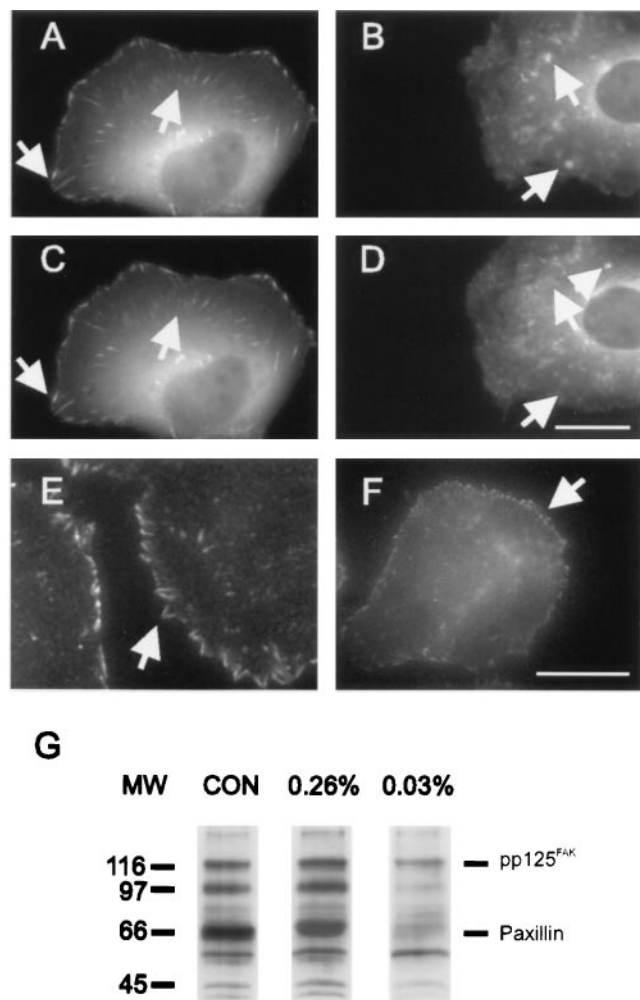
FIG. 3. Distribution of vinculin and phosphotyrosine in NRK cells cultured on substrates with 0.26% bis-acrylamide ( A, C, E ) or 0.03% bis-acrylamide ( B, D, F ). ( A–D ) Cells were injected with rhodamine-labeled vinculin and imaged over a period of 10 min. On more rigid substrates ( A, C ), vinculin is incorporated into elongated focal adhesions, which show only minor changes during the period of observation. On highly flexible gels ( B, D ), vinculin is localized at punctate structures of irregular sizes and shapes, many of which appear and disappear over a period of 10 min (arrows). ( E, F ) Immunofluorescence of phosphotyrosine. Phosphotyrosine is localized at elongated focal adhesions in cells cultured on more rigid gels ( E ), and at punctate structures in cells cultured on highly flexible gels ( F ). ( G ) Anti-phosphotyrosine immunoblotting of whole cell lysates from NRK cells cultured on different substrates. On plastic dishes (CON) and rigid 0.26% bis-acrylamide substrates (0.26%), pp125 FAK , paxillin and a 97-kDa protein are heavily phosphorylated after 48 hr of culture. Cells cultured on soft 0.03% bis-acrylamide substrates (0.03%) show a significantly lower extent of phosphorylation at these bands. Bar = 10 \mu m.
