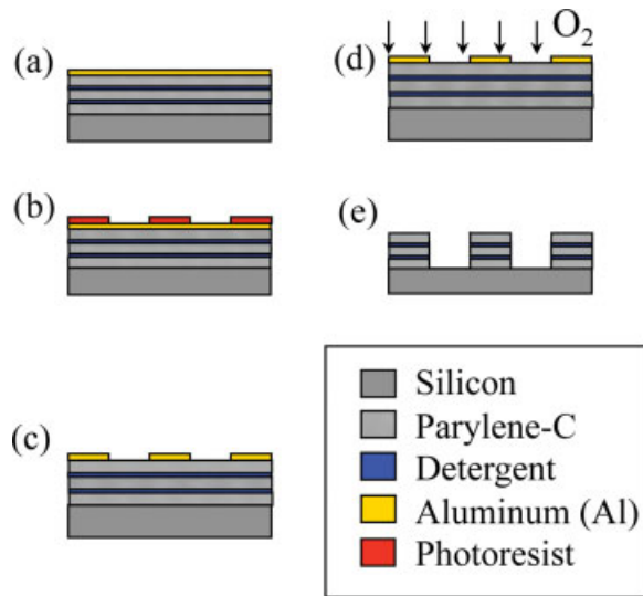
Figure 1. Fabrication process for multilayer parylene-C stencils with a microwell pattern. A thin layer of detergent was applied to each parylene-C layer to generate a peelable multilayer stencil. An aluminum hard mask was deposited on top of the stencil (a). To create the microwell pattern, a thin layer of photoresist was spun and patterned on the substrate (b) and subsequently transferred to the aluminum hard mask by submersing the wafer in an aluminum etchant at 50°C for 1 min (c). Microwell patterns were then generated using low temperature (5°C) dry etching with O 2 plasma (d). After the dry etch process, the aluminum hard mask was removed (e). [Color figure can be viewed in the online issue, which is available at www.interscience.wiley.com .]
