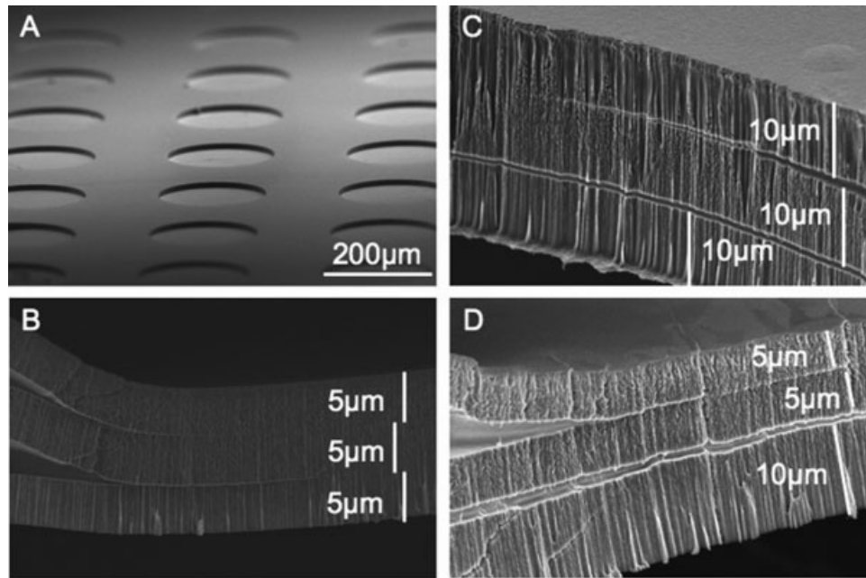
Figure 3. A scanning electron microscope (SEM) image of parylene-C stencils. An oblique view on the top of the stencil displays a pattern of microwells with 200 \mu\text{m} diameter with almost vertical side walls (A). The three-layered parylene-C stencils were engineered with three combinations of layer thicknesses. Cross-sectional images of the stencils were taken at higher magnification to depict the individual layers. The images show three-layered parylene-C stencils with individual film thicknesses of (from top to bottom) 5–5–5 \mu\text{m} (B), 10–10–10 \mu\text{m} (C), and 5–5–10 \mu\text{m} (D).
