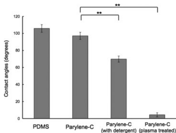
Figure 4. Contact angles for various materials and surface conditions of the parylene-C stencils. The surfaces of the untreated parylene-C stencils were hydrophobic, similar to the PDMS substrate. However, when parylene-C membranes were treated with either detergent or reactive oxygen plasma, their surfaces became more hydrophilic. The contact angle measured for parylene-C was significantly different from angles measured for detergent- and plasma-treated parylene-C (** p < 0.01 ).
