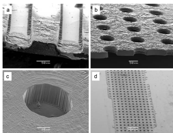
Fig. 2 Scanning electron micrographs of molded PEG lanes (a) and microwells (b–d). The underlying substrate could be either exposed (a) or non-exposed (b) based on the polymer film thickness. (c) Individual patterns of circular microwells demonstrate that the structures are \sim 25 \mu m in height.
